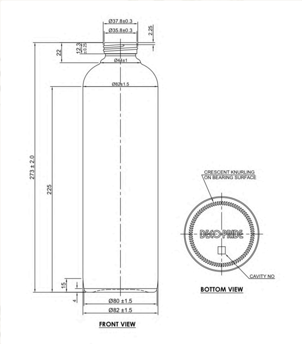
1000ml Water Bottle Mold Design
