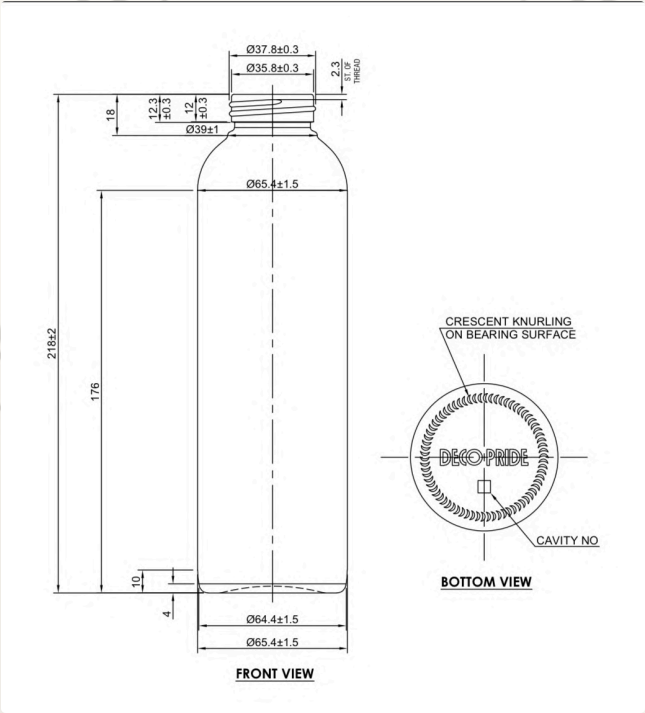
500ml Water Bottle Mold Design
